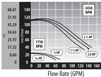
2-SPEED PRESSURE VERSUS FLOW RATE
